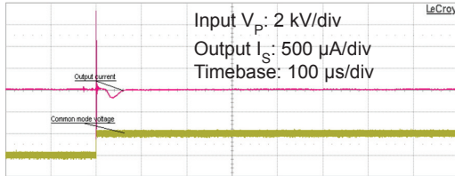
Figure 11: Typical common mode perturbation (2000 V step with 6 kV/µs, R_M = 100 \Omega )
