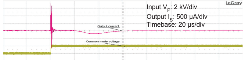
Figure 12: Detail of typical common mode perturbation (2000 V step with 6 kV/µs R_M = 100 \Omega )
